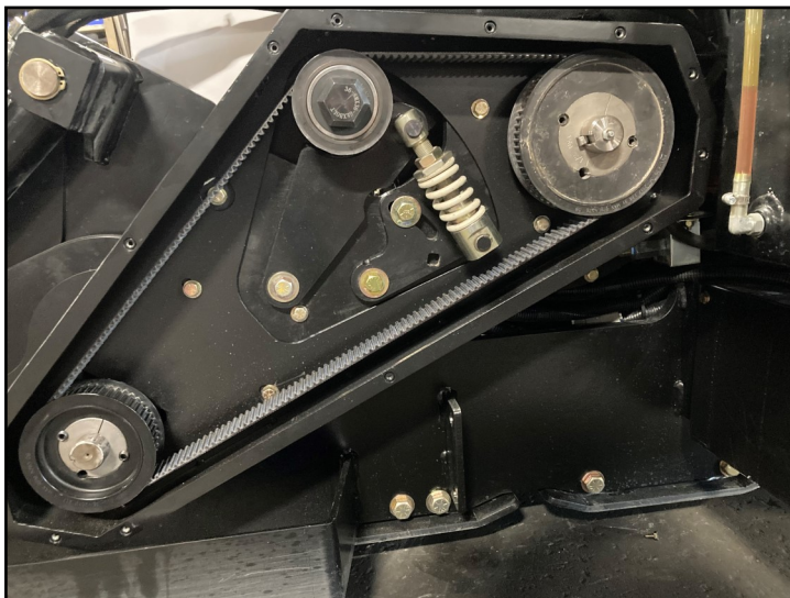
Cutting drum drive with auto tensioner
